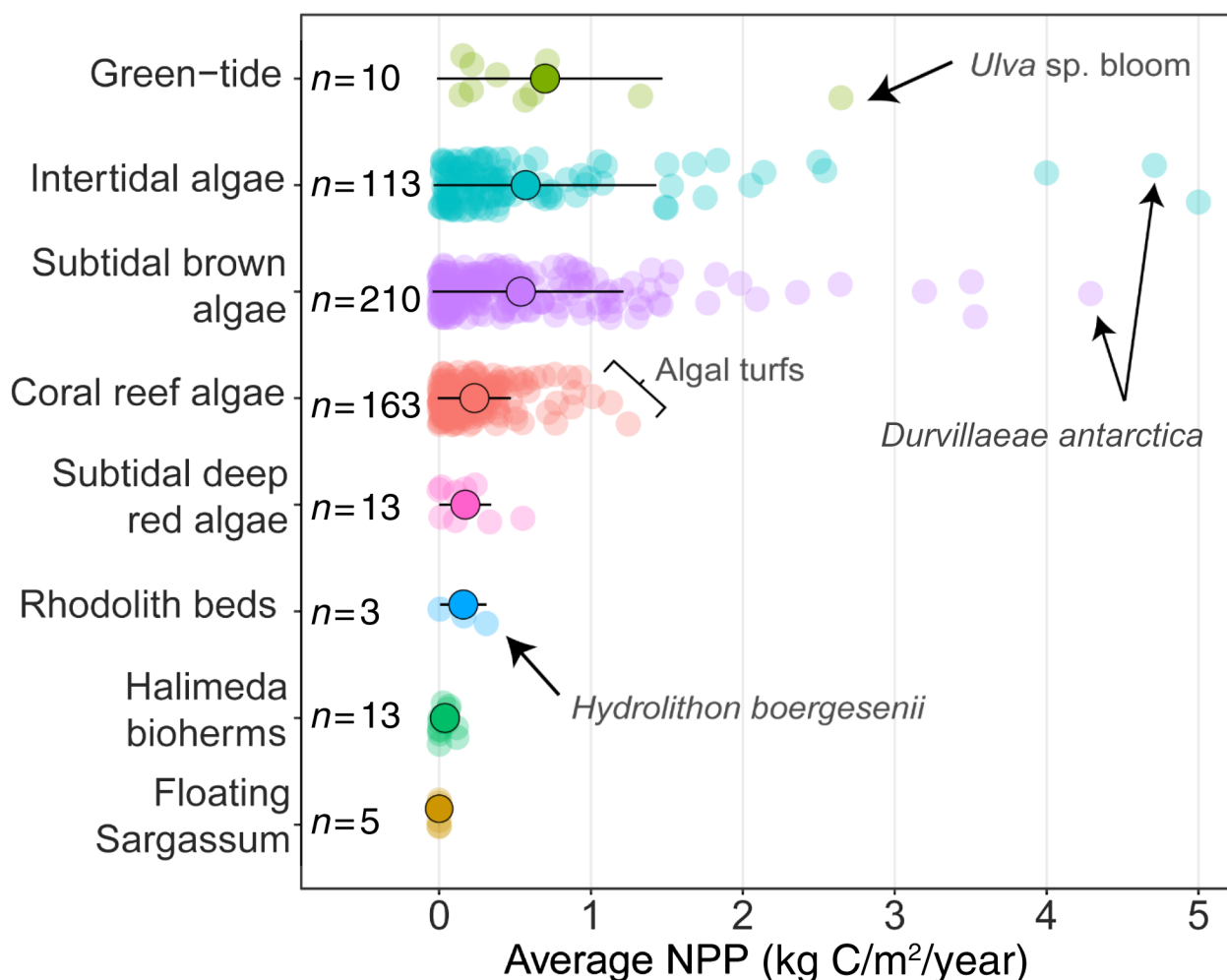
FIGURE 2 Annual net primary productivity for different macroalgal habitat types. Small dots indicate the depth-averaged annual net primary production (NPP) at sites featuring that habitat, while larger dots and error bars indicate the means and standard deviation of each habitat type. The number of site-level measurements for each habitat type is indicated next to each graph (Table 2)
