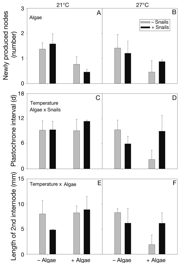
Fig. 4. Halophila ovalis . (A,B) Number of newly produced nodes, (C,D) leaf plastochrone interval and (E,F) length of the 2nd internode (mean \pm SE) for shoots in aquaria with or without algae Chaetomorpha linum and snails Batillaria australis at (A,C,E) 21°C and (B,D,F) 27°C. The factors or interactions named in the graph are those that caused significant differences
