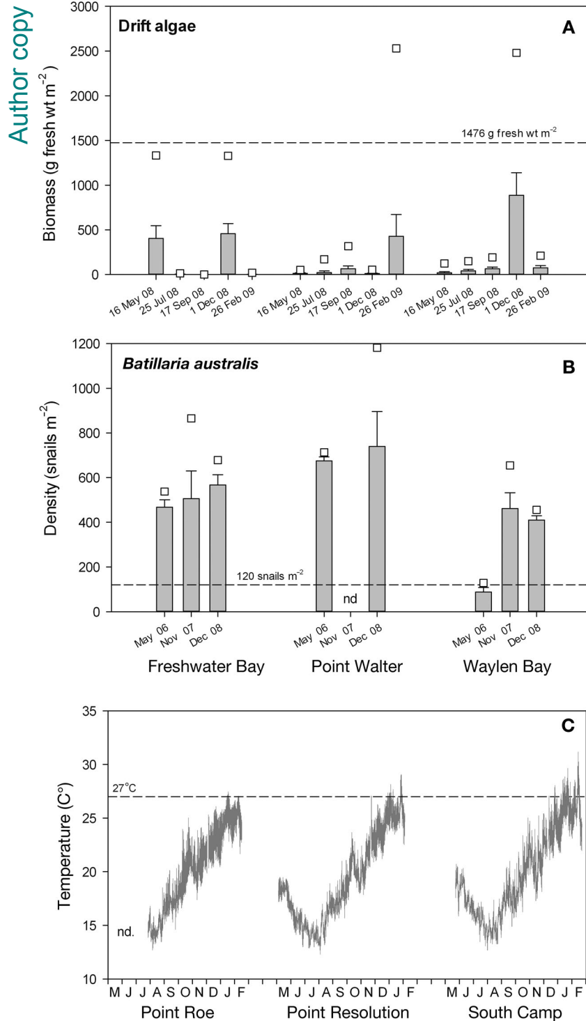
Fig. 2. In situ patterns of (A) biomass of drift algae, (B) densities of invasive snails Batillaria australis and (C) water temperature at 3 sites in the Swan River. Note that (C) shows different sites than (A) and (B). Bars are mean values ( \pm SE) ( n = 10 for drift algae, n = 4 for snails) and white squares are maximum values recorded in any one sample. The dashed lines indicate levels used in the aquarium experiment. nd: no data
